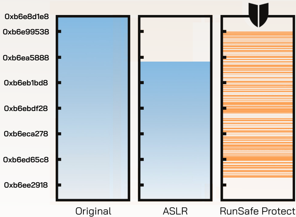
Figure X: Change in memory diversity with Protect's LFR ©RunSafe Security
