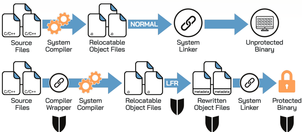
Figure X: Change in build process to add Protect's LFR ©RunSafe Security
